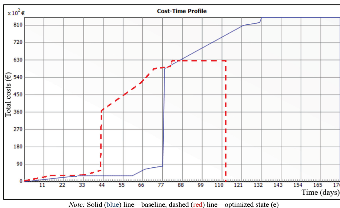
Figure 7. Comparison of the project cost-time profile in the case of a combination of all optimization options and the baseline. Authors own work
