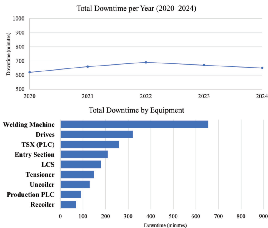
Figure 2. Production line's downtime. Authors own work
